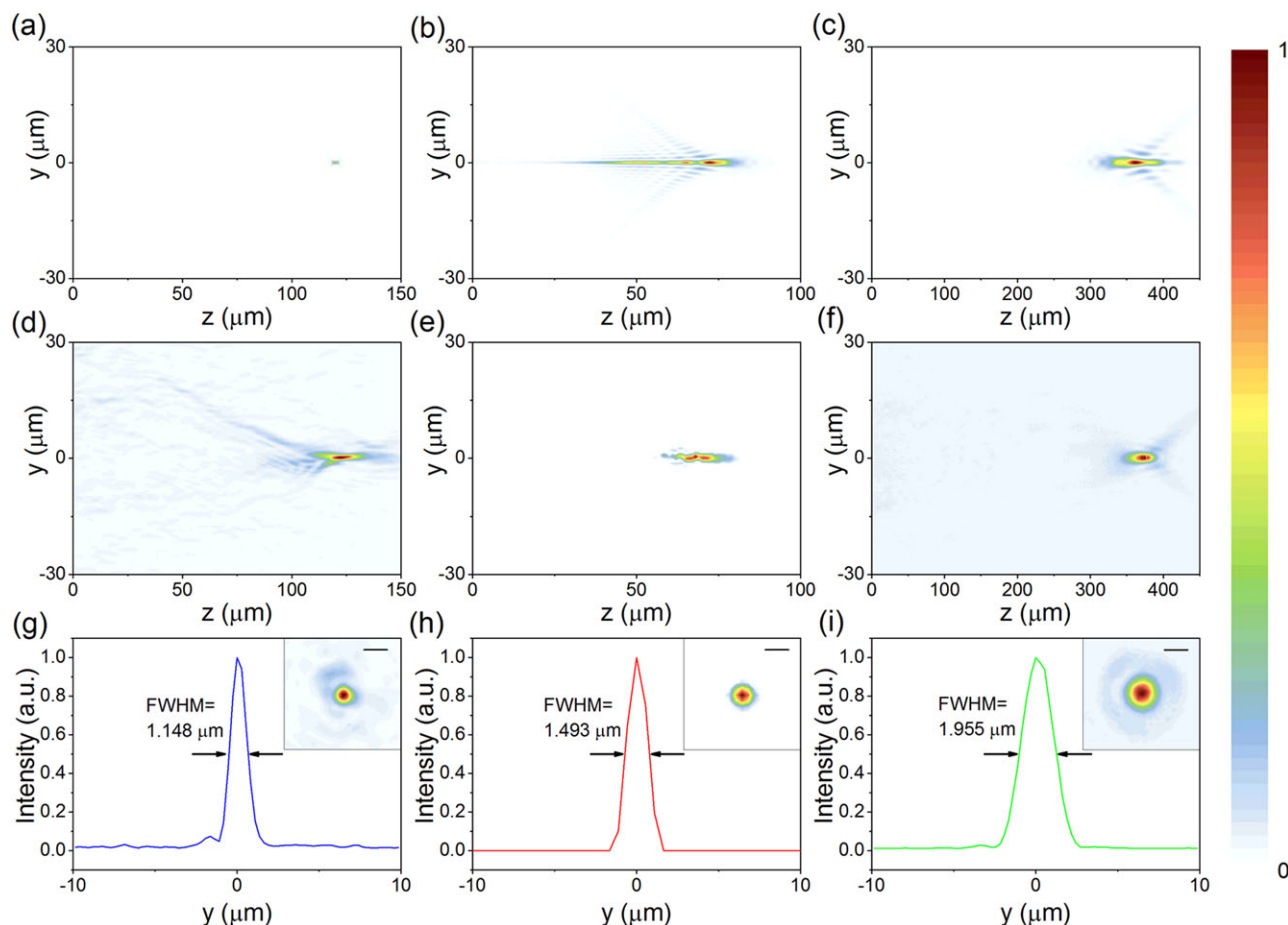
Figure 4. Calculated and experimental intensity profiles of the metalens. a–c) Numerically calculated intensity profiles for THG (a), FF (b), and SHG (c) in the y–z plane. d–f) Experimentally measured intensity distributions for THG (d), FF (e), and SHG (f) in the y–z cross section. The center of the metalens is taken as the origin in (a–f). g–i) The experimentally measured intensity distributions of the focal spots along y-axis for THG (g), FF (h), and SHG (i). The insets in (g–i) represent the measured intensity profiles of x–y cross sections at the focal planes (scale bar: 2 μm).
