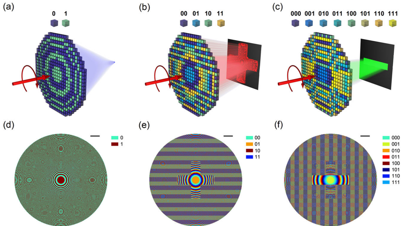
Figure 5. Schematic diagrams and coding patterns of the designed multifunctional metasurface. a) The focusing procedure for the THG channel. b,c) The reconstruction procedures of the operational symbols “+” of the FF channel (b) and “−” of the SHG channel (c). Only the schematic distributions of digital elements are shown on the sample surfaces in (a–c). d–f) The coding patterns of multifunctional metasurface for the THG (d), FF (e), and SHG (f). The scale bars represent 20 \mu\text{m} .
