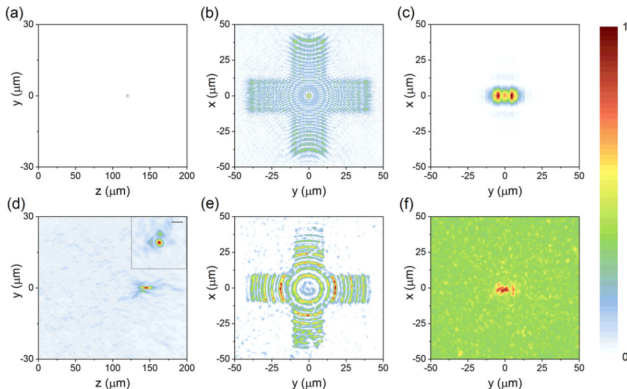
Figure 6. Calculated and experimental intensity profiles of the nonlinear coding multifunctional metasurface. a) Calculated intensity profile for THG in the y-z plane. b) Numerically calculated real space image under the FF channel. A perfect symbol “+” is obtained in the far field. c) Numerically calculated image under the SHG channel. A focused symbol “—” is achieved in the relatively far field. (b) and (c) show the calculated real space images in the x-y plane. d–f) Measured results corresponding to (a–c) for the multifunctional metasurface. The inset in (d) represents the measured intensity distribution of focal spot at the focal plane (scale bar: 2 \mu\text{m} ).
