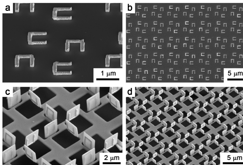
Figure 2. Experimental demonstration of toroidal metamaterials. a,b) SEM images of SRR arrays on planar SiN x film in 52° tilted view and top view, respectively. c,d) SEM images of toroidal metamaterial array in 52° tilted view.
